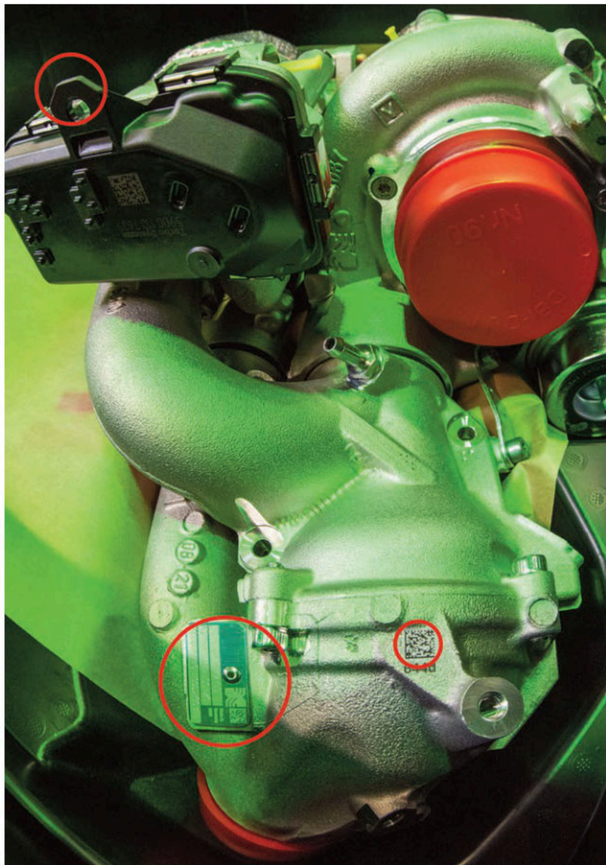
Twelve features of a turbocharger assembly are inspected from 3.5 m above. Circled in red are a 3 mm-wide plastic web, the assembly's nameplate and a small 5 mm × 5 mm DataMatrix code.
